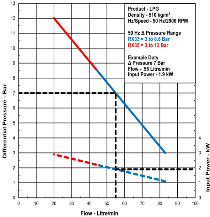
RX33 and RX35 - 50 Hz Performance
