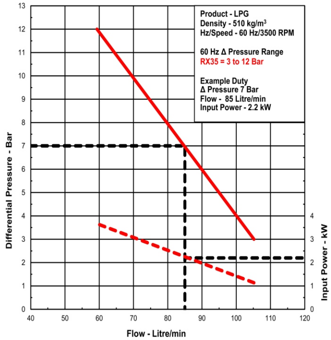
RX35 - 60 Hz Performance
