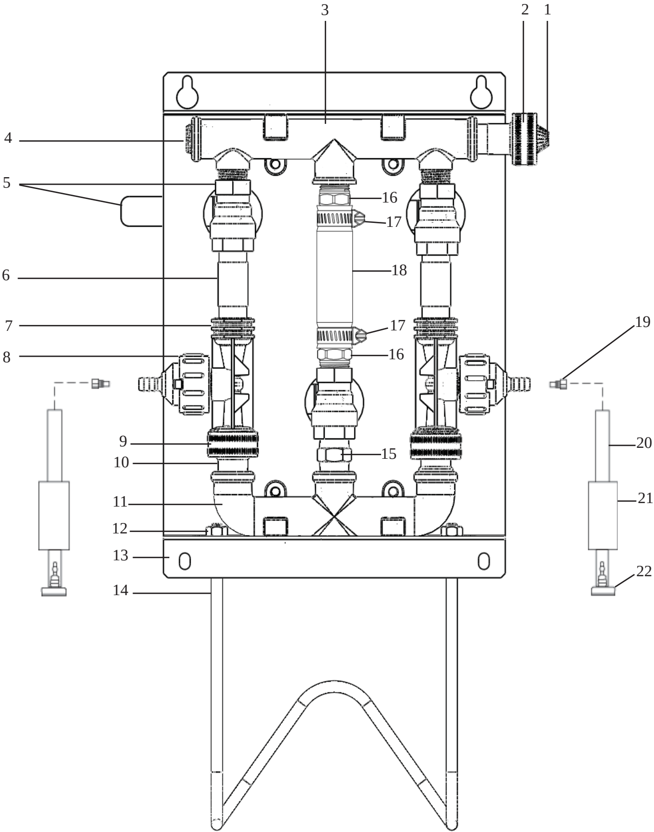
HydroChem Parts Diagram:
