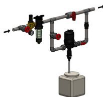
By-pass installation
