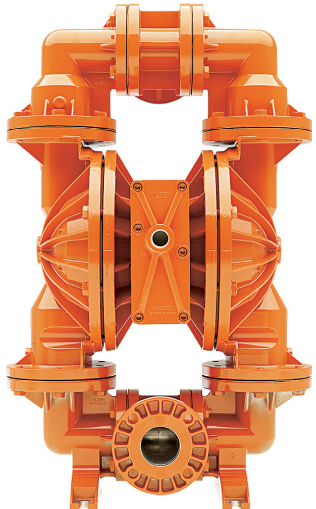
Wilden® Advanced™ Series Metal PX1500 AODD Pump
